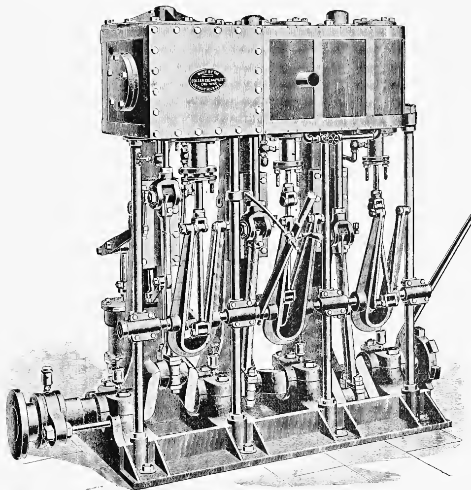
THE COLLIER YACHT ENGINE.—Designed by B. J. Collier, Detroit, Mich.
